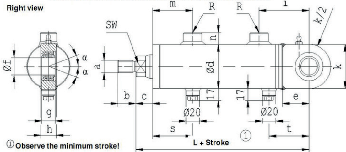
Double-Action Damping Cylinders - 210 bar Series: HZD4 Model: A Position of the P5 and P6 vents and the P7 and P8 connections
